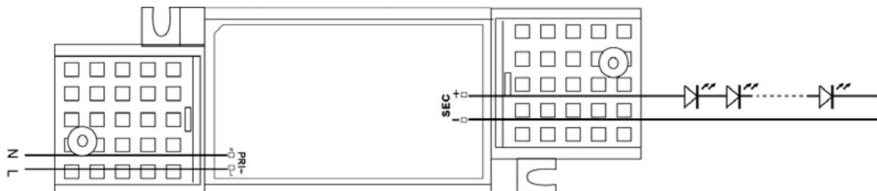
1600420 DCC TRIAC 20W 350-500mA
